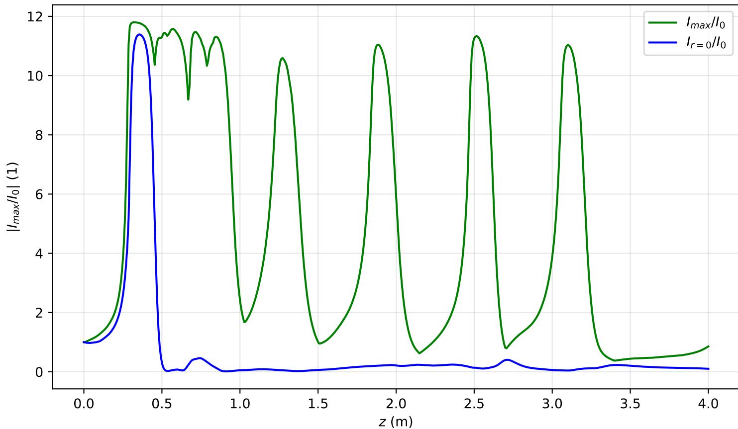
I_{max}(x=0, y=0, z)/I_0 , \text{Pin}=9.4\text{Pcr} , noisy input, artificial time
